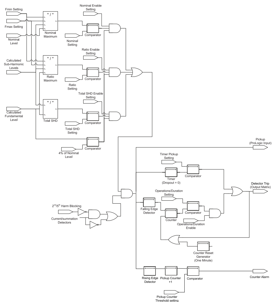
Figure 5.6: Sub-Harmonic Measurement and Detection Logic
