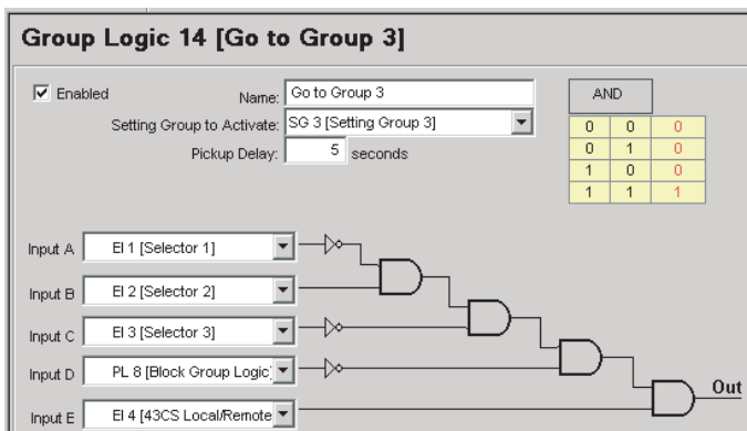
Figure K.9: Group Logic 14
