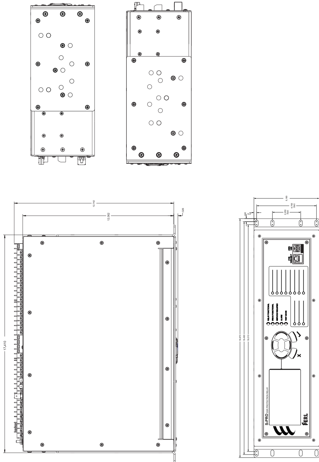
Figure G.1: Mechanical Drawing (3U)
