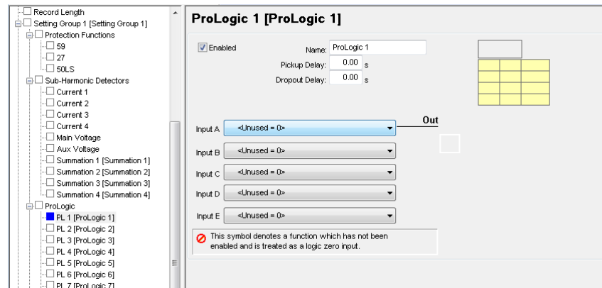
Figure 7.20: ProLogic
