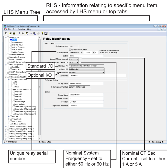
Figure 7.3: Relay Identification
