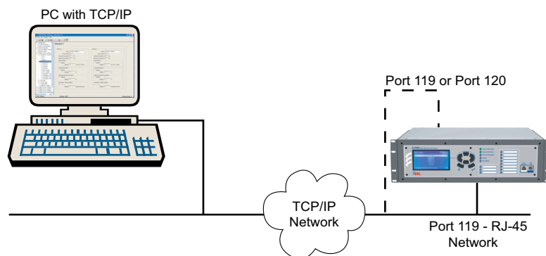
Figure 3.2: Network Link
