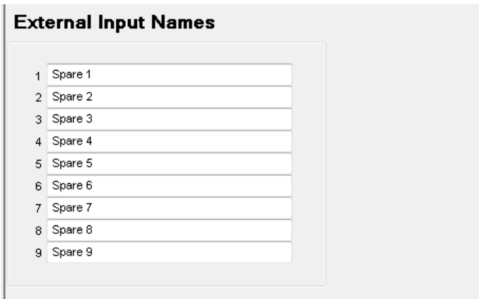
Figure 7.5: External Inputs
