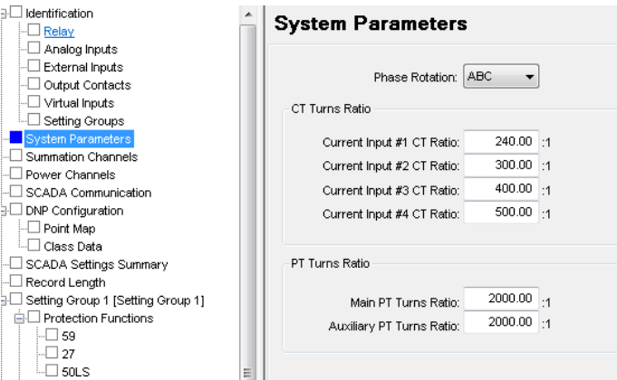
Figure 7.11: System Parameters
