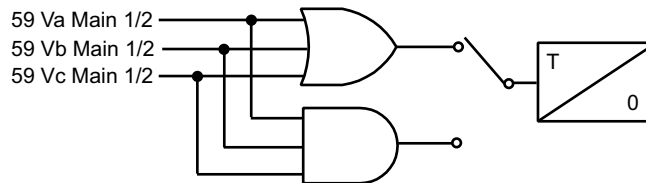
Figure 5.9: 59 Main Overvoltage Logic
