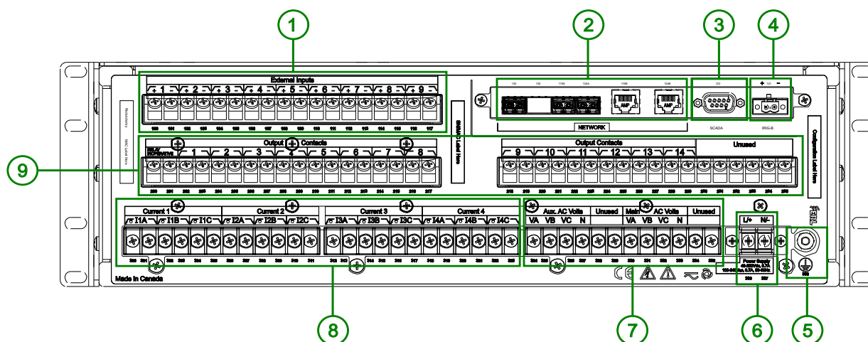
Figure 1.3: S-PRO Relay Rear View. LAN Port Configuration: Options 1, 2 and 3 (with redundancy)
