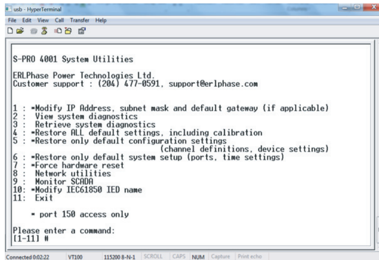
Figure 6.6: Maintenance Interface
