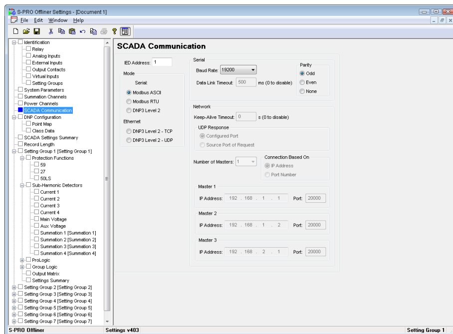
Figure 6.3: SCADA Communications
