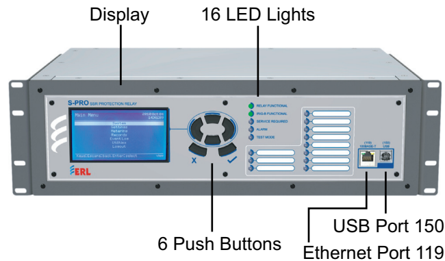
Figure 4.1: Front Panel Display
