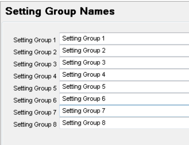
Figure 7.10: Setting Groups
