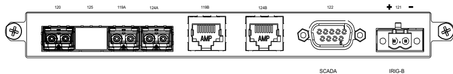
Figure 3.7: Redundant Communication Ports
