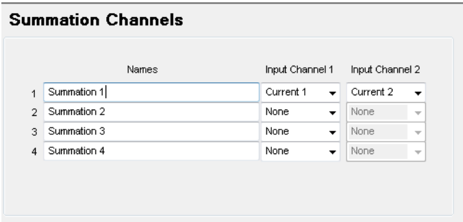
Figure 7.7: Summation Channels
