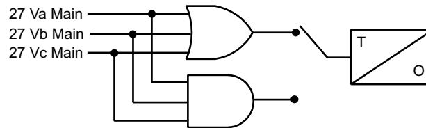
Figure 5.8: 27 Undervoltage Logic
