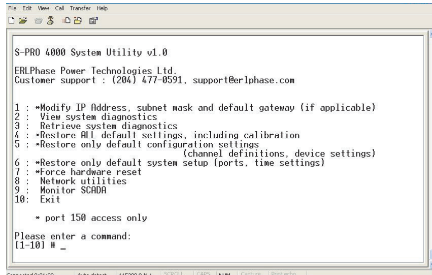
Figure 3.6: Maintenance Menu
