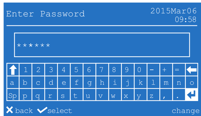
Figure 4.4: Enter Password
