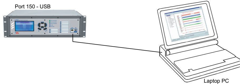
Figure 3.1: USB Link
