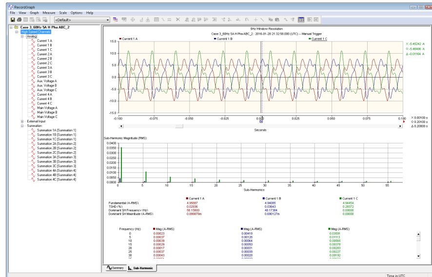
Figure 7.23: RecordGraph
